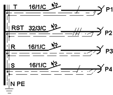
SCHEMA MONOFILARA
